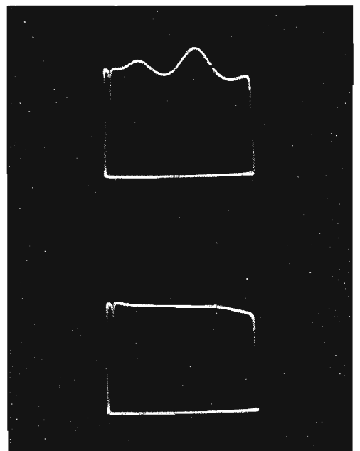
FIG. 11. Sweep frequency response of 75 feet of RG-11/U terminated at the receiving end with 75 ohms shunted with 100 mmf. This is a typical input capacity for switches and paralleled bridge inputs. The upper curve was obtained by feeding the cable with an amplifier with high impedance output (TA-1A). A TA-3A, which provides a good termination at the sending end of the line, was used for the lower curve. Note the uniform response obtained with the TA-3A as a result of minimized reflections. Marker is at 8 megacycles.
