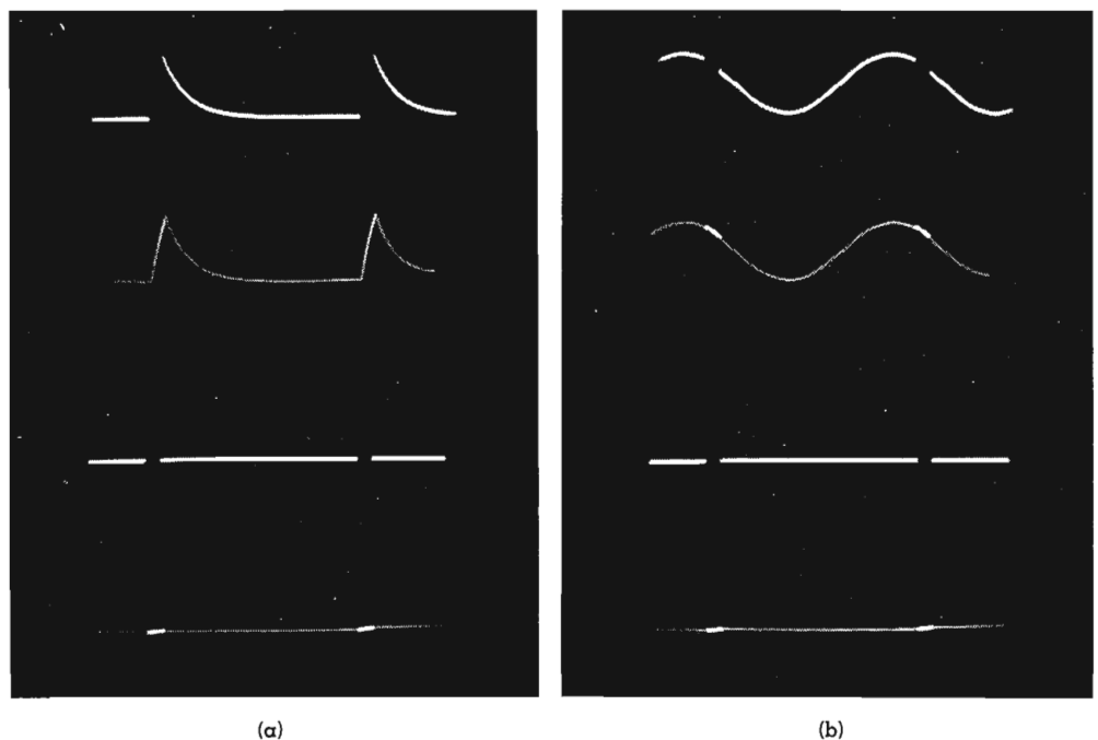
FIG. 6. Defects frequently encountered with pulse signals are tilt and 60 cycle hum. Waveforms at (a) show elimination of tilt, and in (b) removal of a hum component from blanking.
