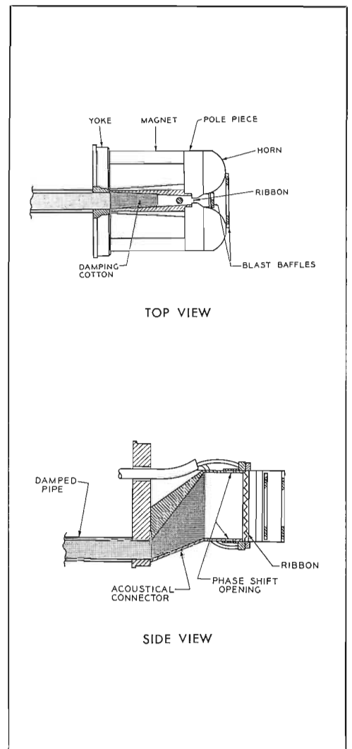
FIG. 8. Cutaway view of BK-5A.
