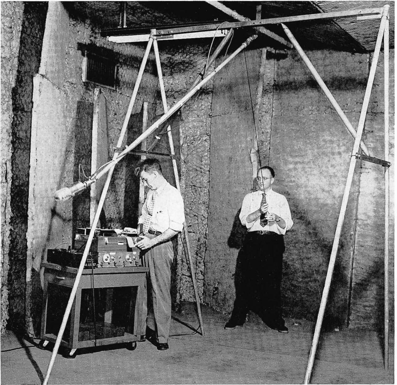
FIG. 1. Producing a standard, controllable quiet wind by use of a pendulum device in the transducer design laboratories at the RCA Camden Plant.
