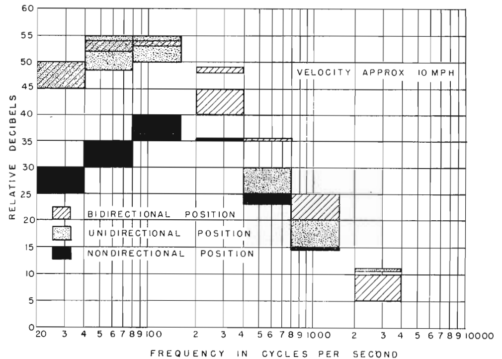
FIG. 2. WIND NOISE SPECTRA OF TYPE 77D MICROPHONE
