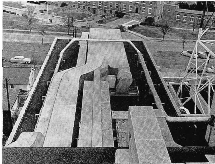
FIG. 13. Air conditioning ducts are very large. Some were placed on roof to conserve interior space.
