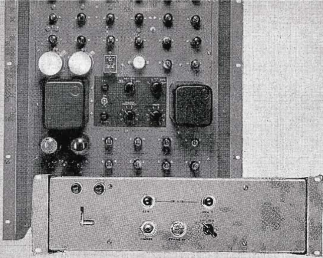
NEW STUDIO SYNC GENERATOR TG-2A (Field Generator is Type TG-12A). Combines sync generator, dot generator, Genlock, grating generator, regulated power supply—on a single chassis. Automatic Changeover Switch MI-26289 (illustrated) is a companion unit for convenient switching between two sync generators.
