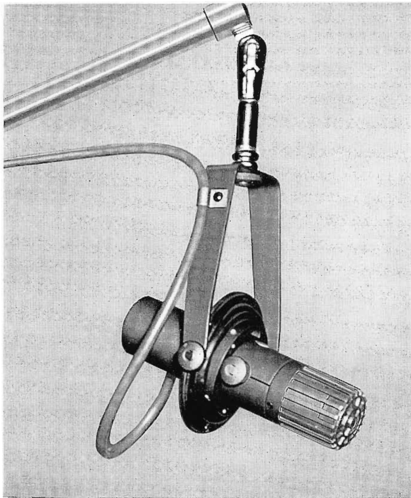
FIG. 1. The BK-5A is an excellent microphone for TV boom operation. New and improved shock mount affords simple, reliable, noise-free handling.
