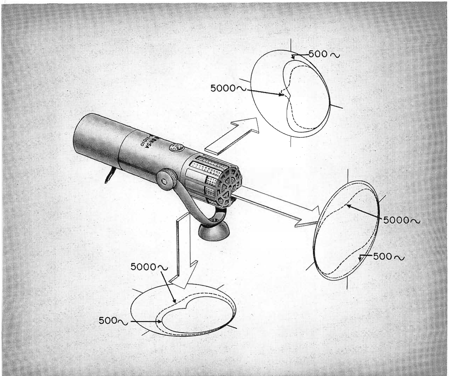
FIG. 3. Perspective view of the BK-5A showing the high frequency and low frequency directional characteristics about the major axes. At low frequencies, the pickup pattern is a true cardioid. At 5000 CPS and above, the pattern becomes fan shaped. This can be utilized to reduce pickup of scraping noises from the floor of a television set. The direction patterns shown in above sketch are illustrated in more detail in Fig. 7.
