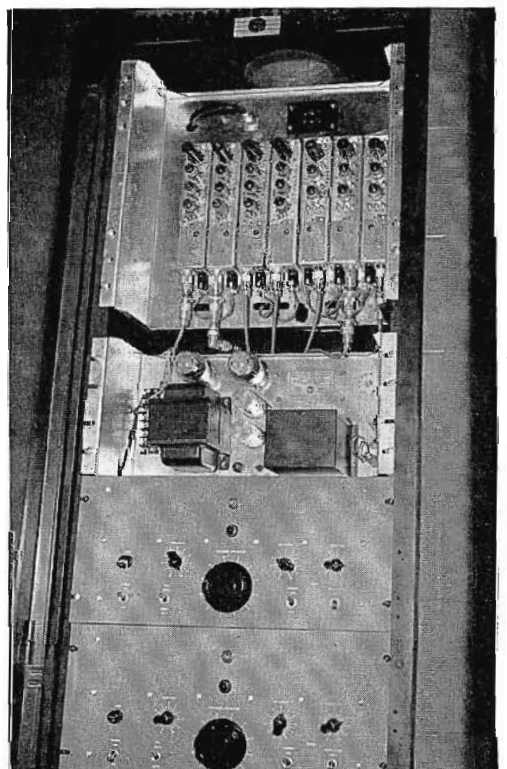
FIG. 33. "Antenaplex" strip amplifiers and monitors, rack mounted in equipment room adjacent to television master control.
