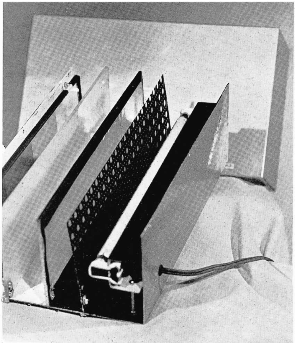
FIG. 2. The grey scale monitor consists essentially of a fluorescent light source modified by a filter and diffusing material. Interior view is shown here. Construction details are given in text.
