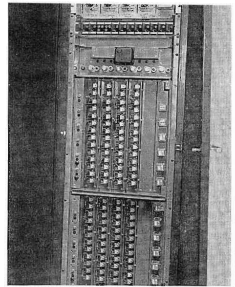
FIG. 22. Control room rack showing TS-20A video relays, distribution and mixing amplifiers.
