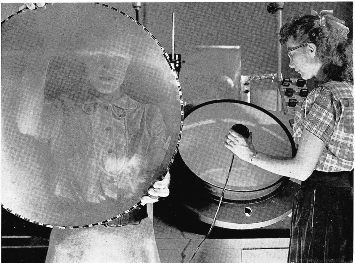
FIG. 2. RCA 21-inch round metal color television picture tube in production at the RCA Tube Division plant in Lancaster, Pennsylvania. Operator at right is directing an ultraviolet source on the faceplate of a color kinescope to "excite" color phosphors for examination of the screen. At left, another operator inspects the tube's shadow mask which contains more than a third of a million accurately-positioned holes. The mask is made of cupro nickel, .0075 inches thick. Holes are accurately etched from both sides of the sheet to produce sharply defined holes of approximately 10 mils diameter. The mask is drawn to spherical shape, plated and blackened, and mounted on a stabilized ring of cold rolled steel.
