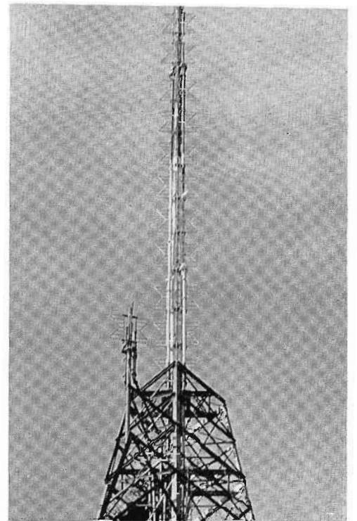
FIG. 28. The emergency single-bay antenna has the same height as the tower (300 feet). The overall height of 12-bay antenna is 783 feet above sea level and 373 feet above ground.
