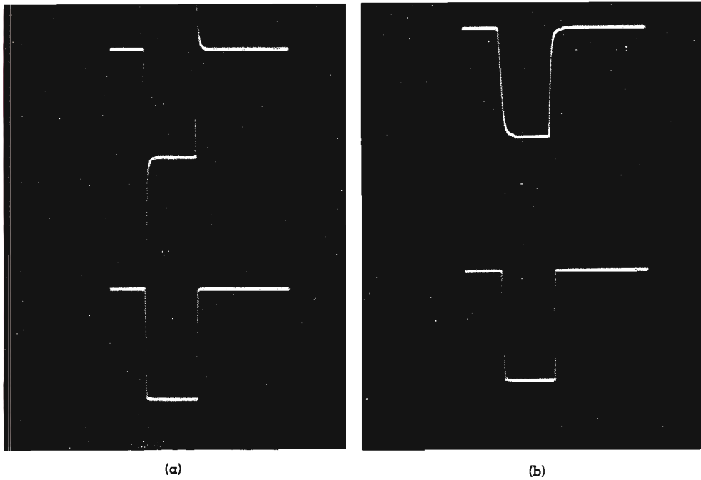
FIG. 7. Waveform photographs showing the effectiveness of the TA-4A in removing overshoot (a), and restoring rise time (b). Regenerated horizontal drive at output is shown at bottom of photographs.
