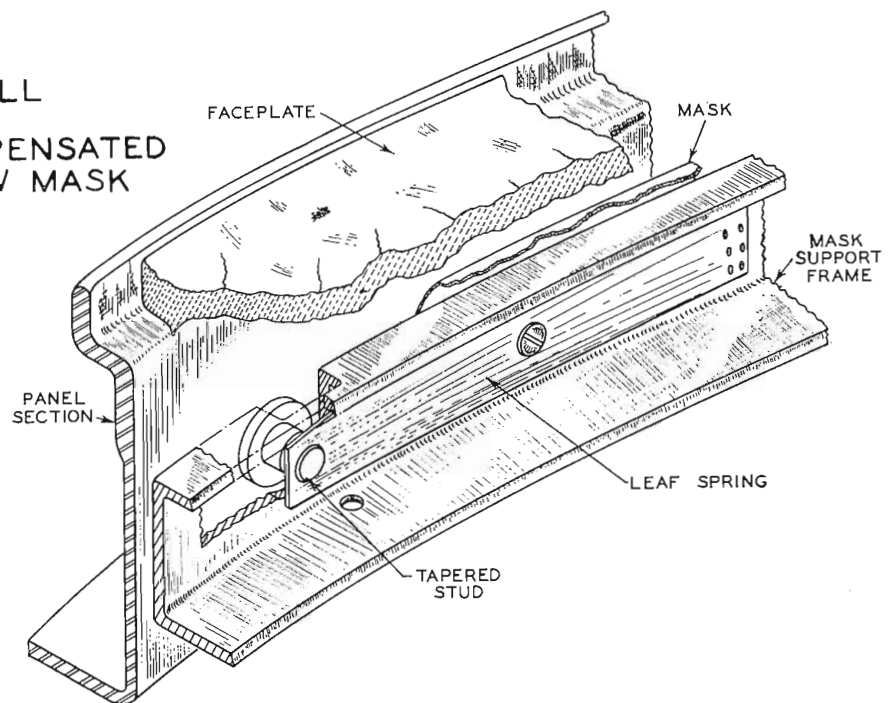
FIG. 5 (right). Cutaway drawing showing the method used to mount the mask assembly in the panel section of the metal tube shell. The entire assembly is suspended on the ends of three leaf springs which have holes fitted over the ends of tapered studs. This mounting arrangement allows the mask assembly to move and expand during the high-temperature exhaust cycle and then return to its original position when the tube reaches room temperature. The development of this method of mounting the mask assembly overcame one of the most serious problems in the production of shadow mask tubes.
