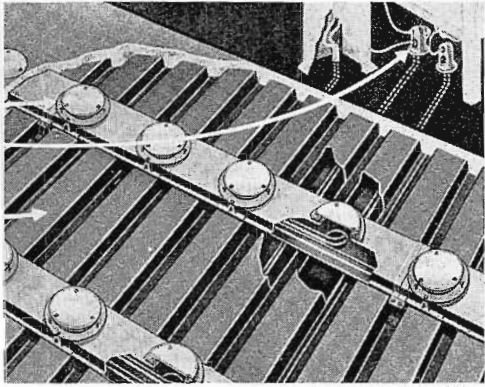
FIG. 10. Q-floor installation similar to that used throughout the building.
