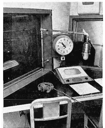
FIG. 36. Television Studio No. 12 announce booth showing clock and monitors. All announce booths are equipped with the same facilities.
