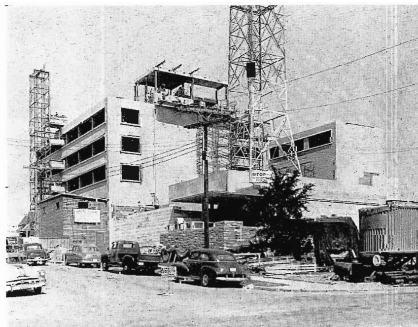
FIG. 6. One-and-one-half years were required to build the new building and to integrate it with the one-story transmitter building.
