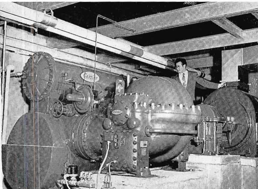
FIG. 11. Four-hundred-ton Carrier compressor for air conditioning.
