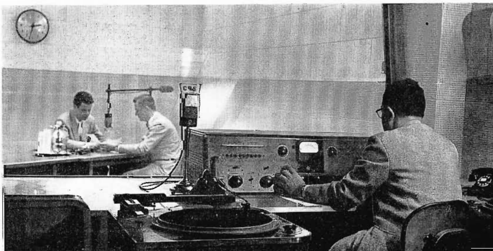
FIG. 39. The operating position in Studio 4 sub control room affords 100 per cent visibility into the studio. The RCA 76 consolette dominates this scene. The nearby 70C turntables and the extended control panel lends to the ease of operation.
