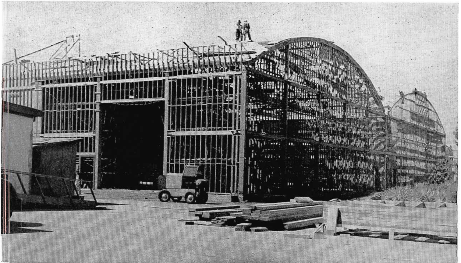
FIG. 2. Multiple sound stage building under construction.
