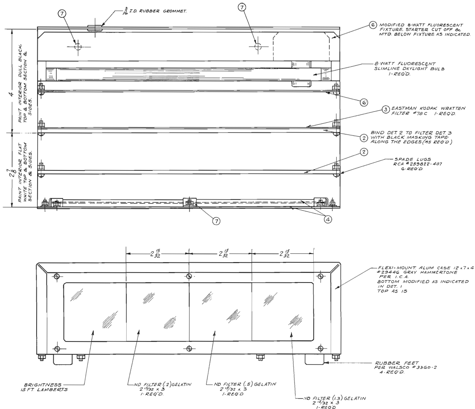
FIG. 3. Assembly of the "Illuminant C" Grey Scale Monitor is shown in this drawing. Numbers in circles refer to detail drawings on opposite page.
