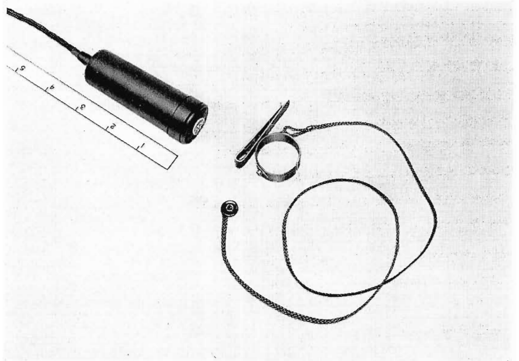
FIG. 4. Size is compared to an inch scale. Also shown are clip and lanyard for versatile mounting.
