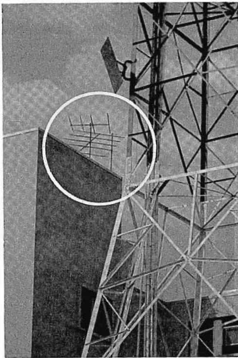
FIG. 32. View of receiving antenna for "Antenaplex" system.
