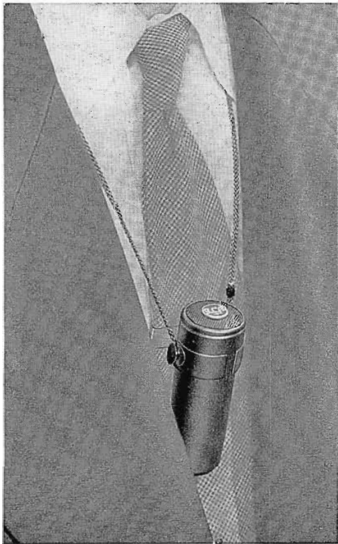
FIG. 2. BK-6A Microphone used as "necktie" mike. May be mounted beneath the necktie or exposed.
